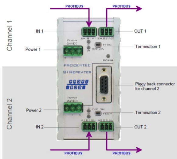
PROFIBUS DP repeater B1
