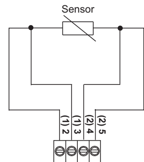
4-Leiter 4-wire
