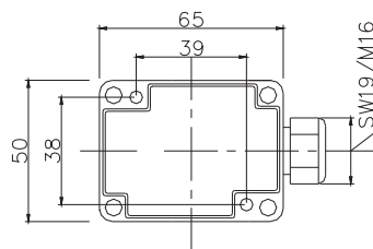
AGS 54 Sensor
