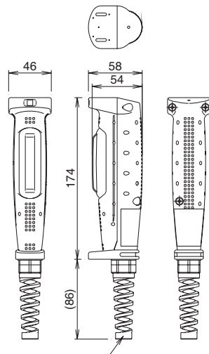
Cable Gland (supplied with grip style enabling switch) Part No.: SKINTOP BS-M20 × 1.5 (LAPP)
