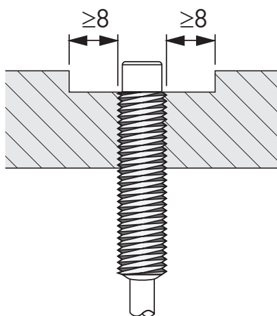
Non-flush mounting
